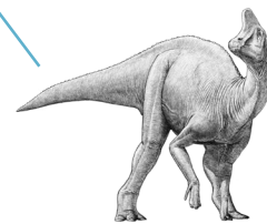
Hadrosaur
