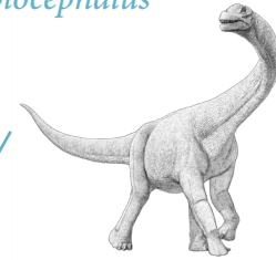
Camarasaurus
